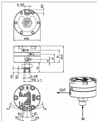
Fig. 5: Dimensions
