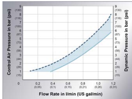
Fig. 3: Characteristic curve of the outflow rate
