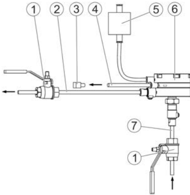
Fig. 2: Assembly drawing (example)
