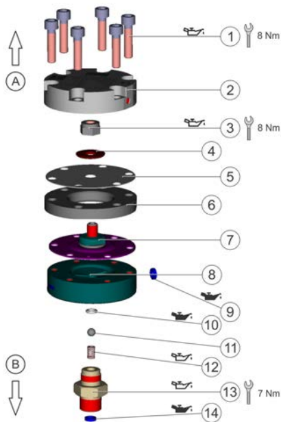
Fig. 4: Exploded view
